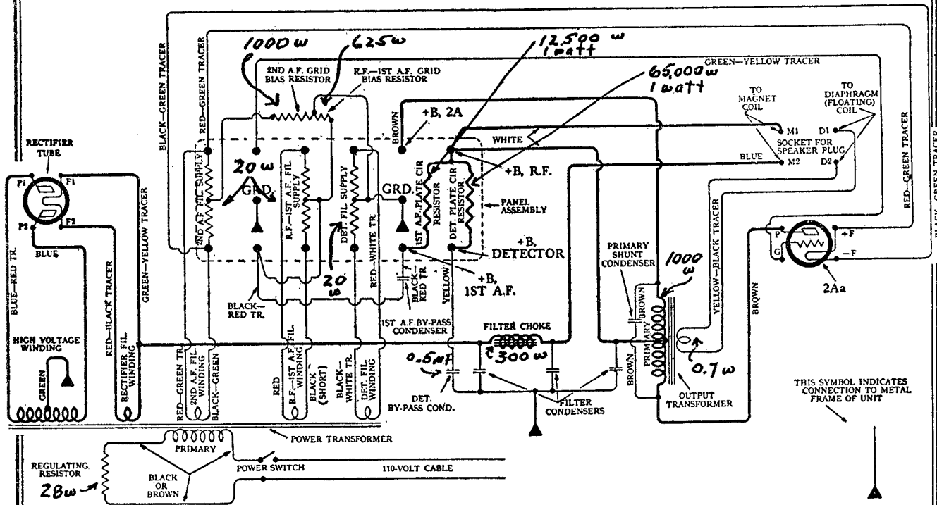
WIRING DIAGRAM OF POWER UNIT IN MODEL 43.
